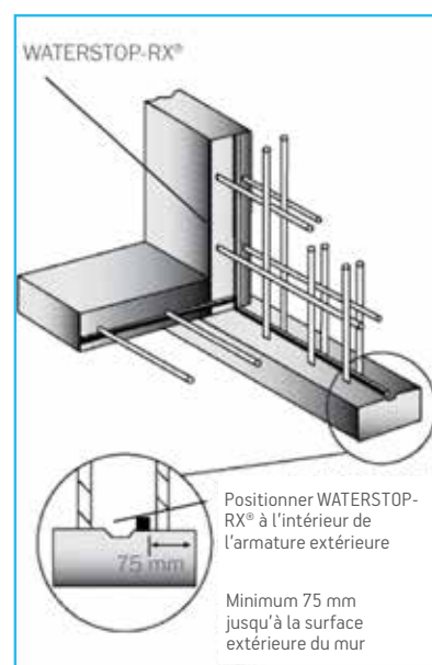
Raccord fondation/mur
