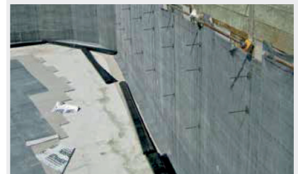
Vertical installation
