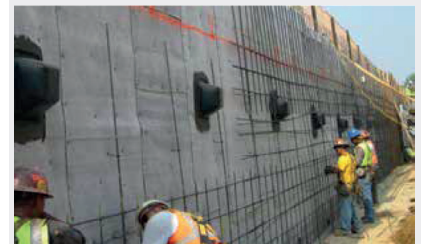
Vertical installation
