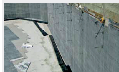
Vertical installation
